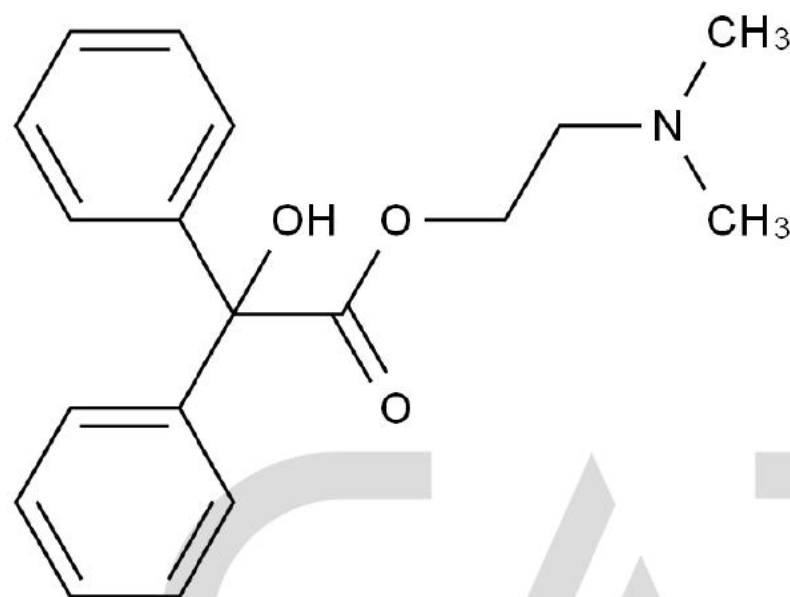
Chemical Structure:
