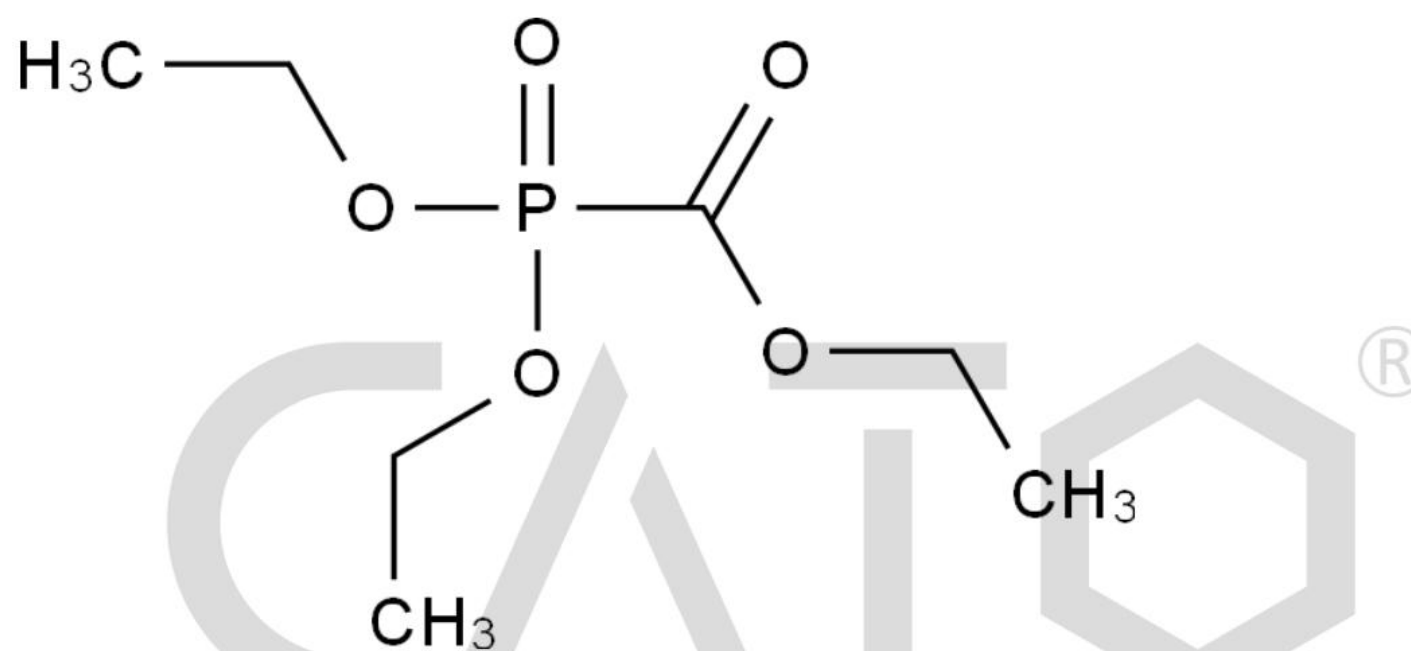
Chemical Structure:
