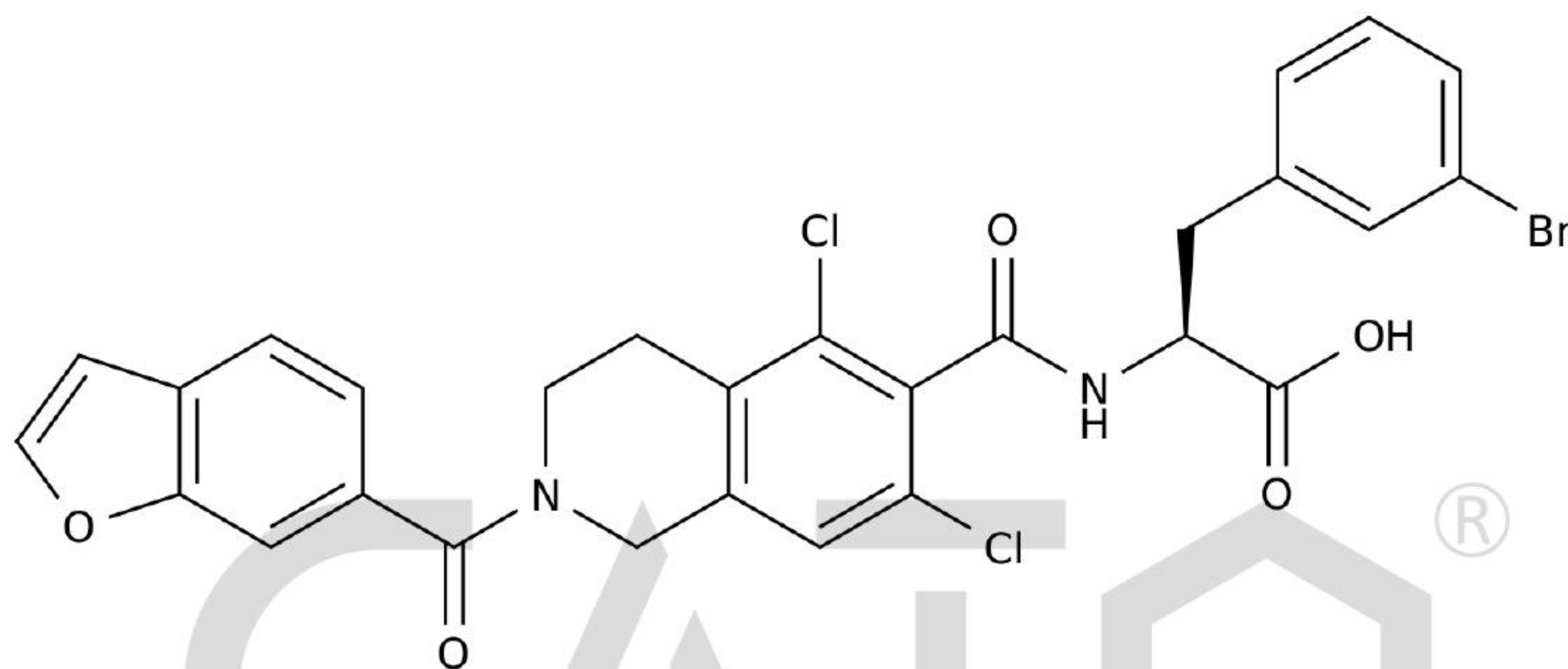
Chemical Structure:
