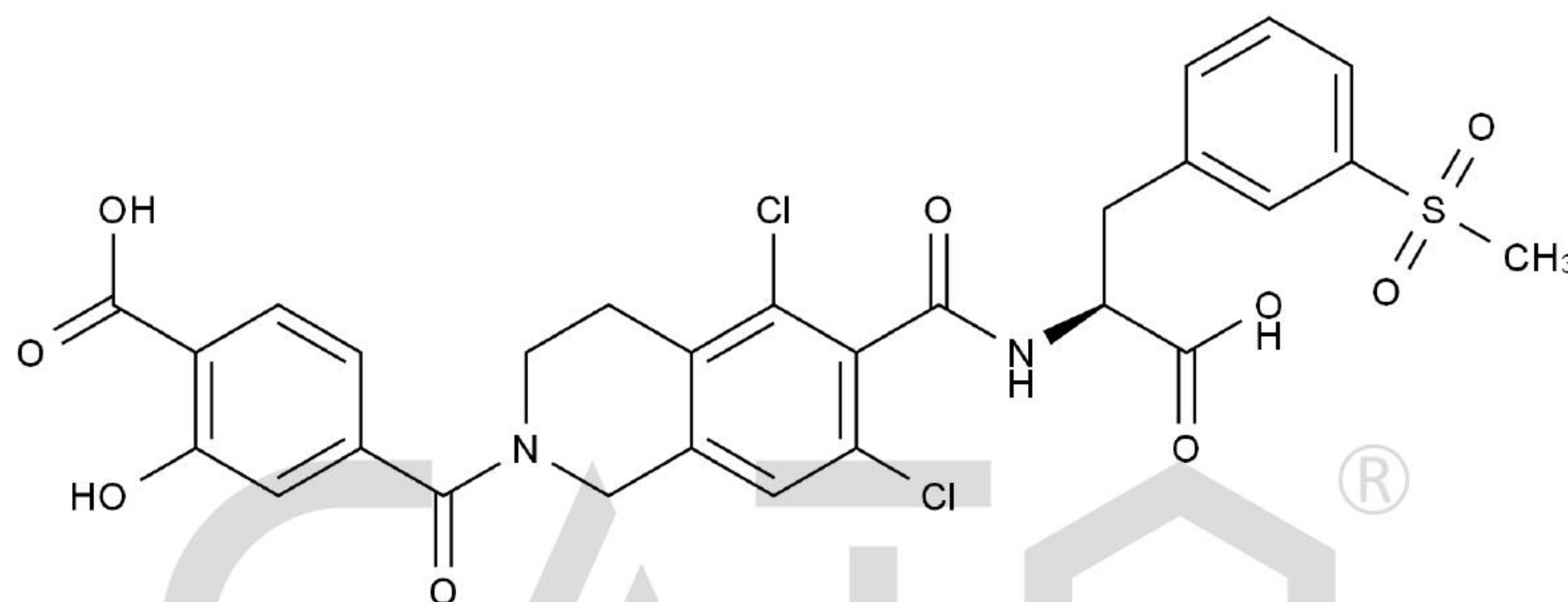
Chemical Structure:
