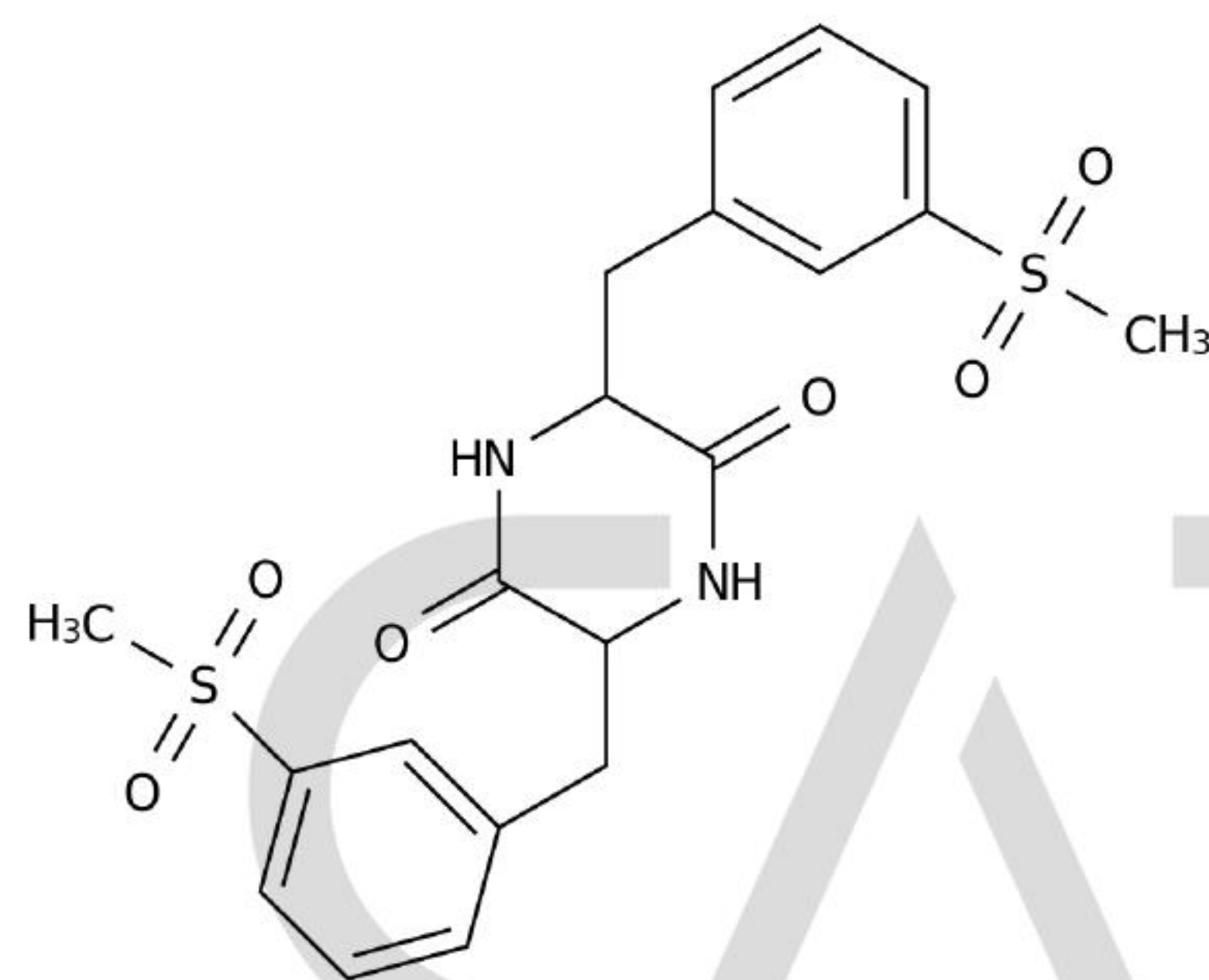
Chemical Structure:
