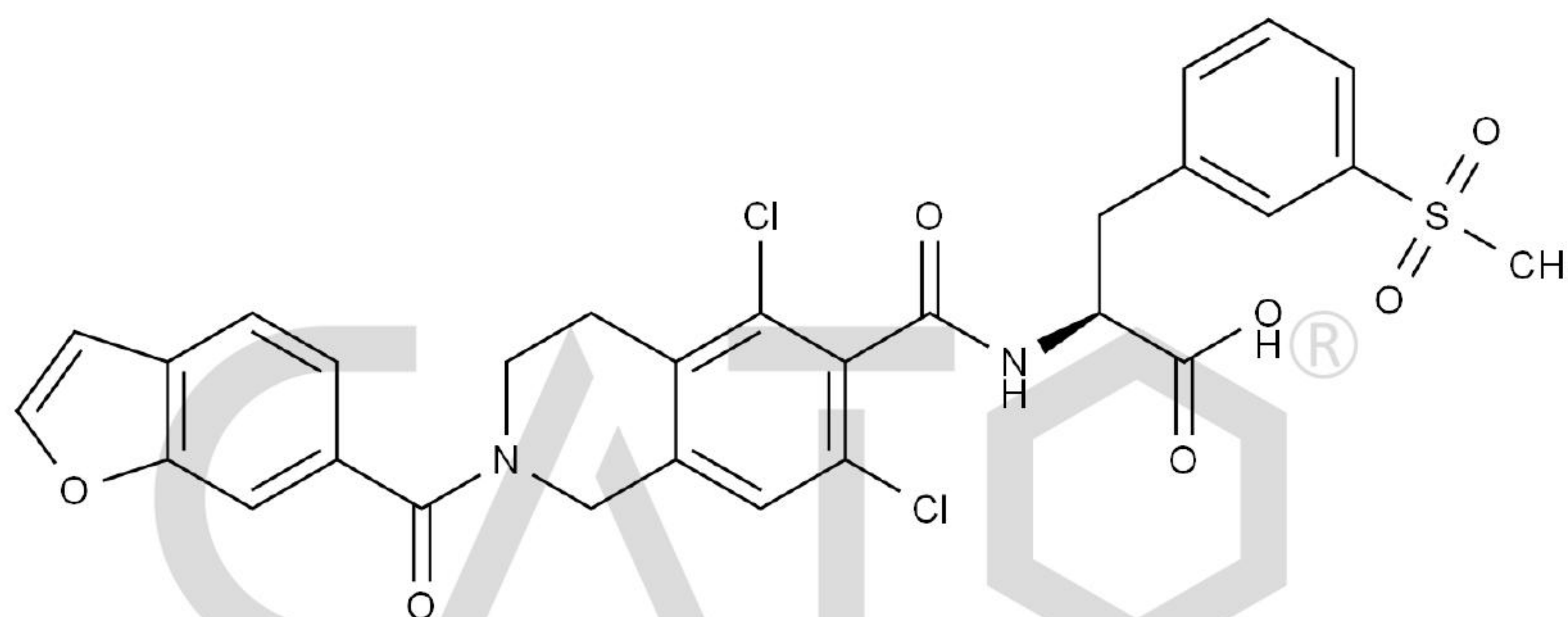
Chemical Structure:
