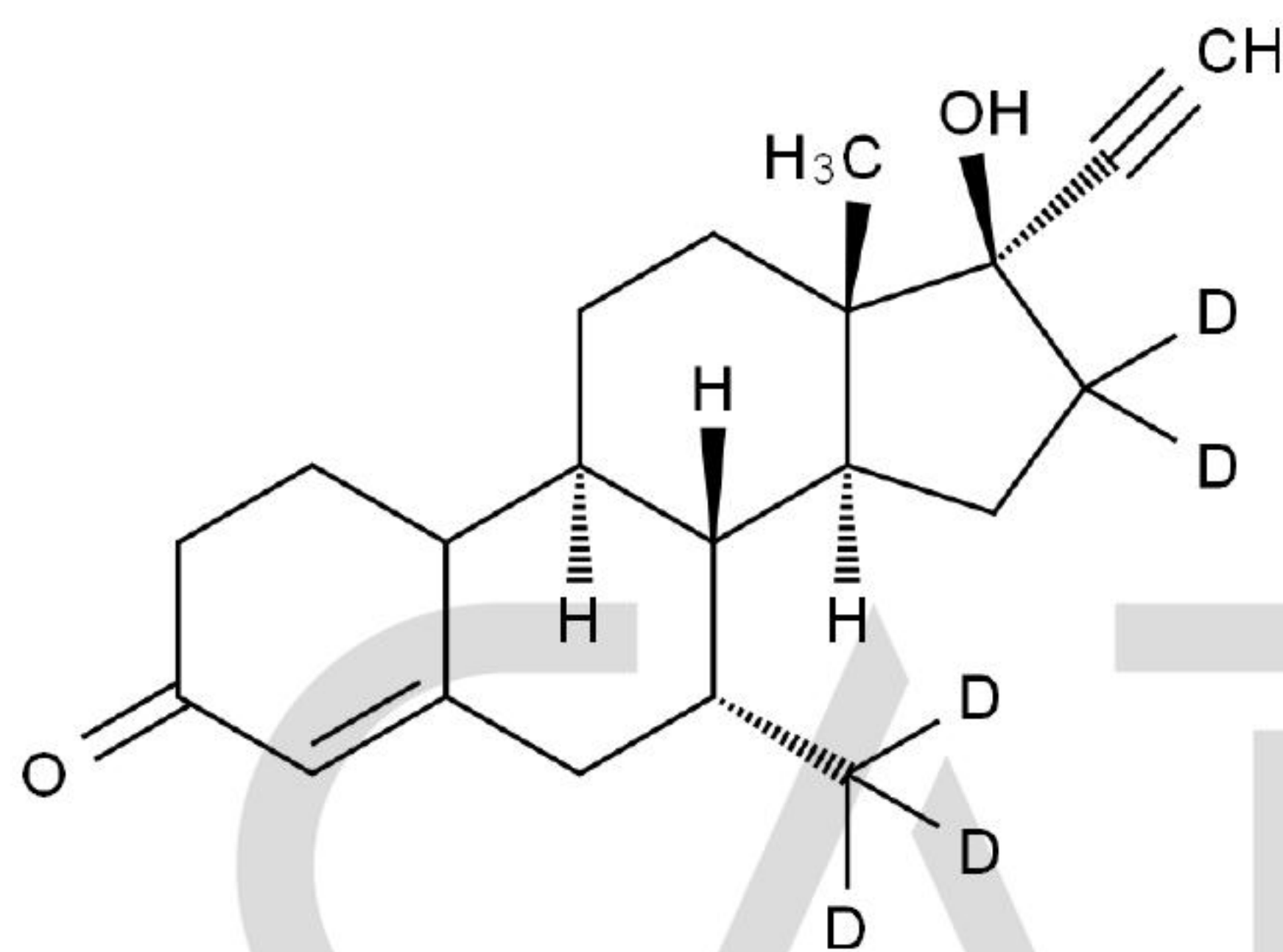
Chemical Structure:
