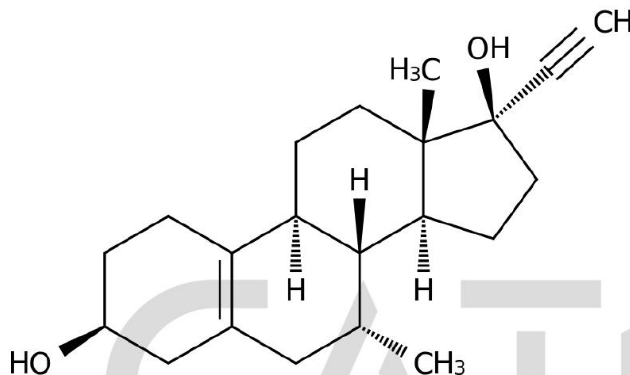
Chemical Structure:
