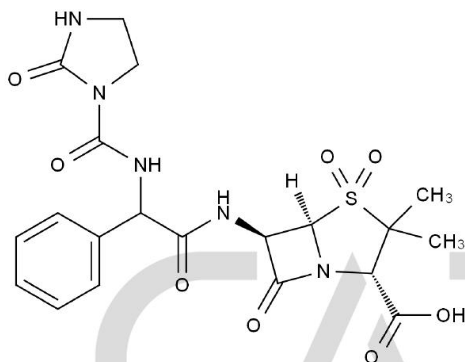
Chemical Structure:
