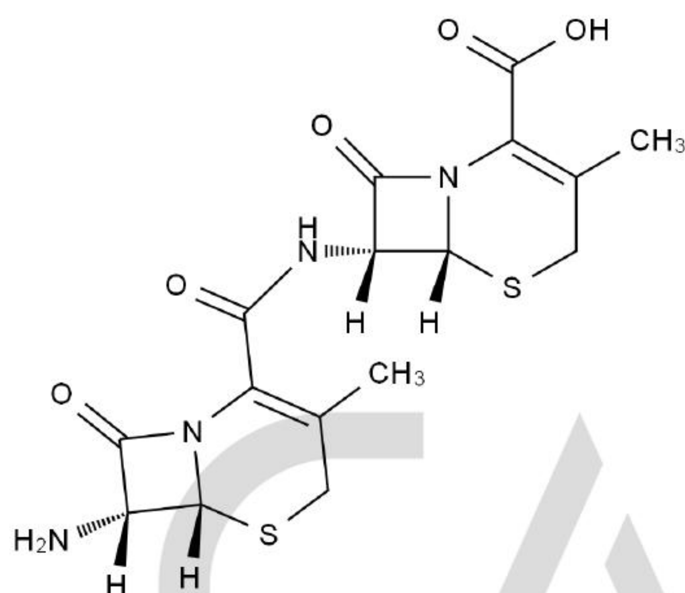
Chemical Structure:
