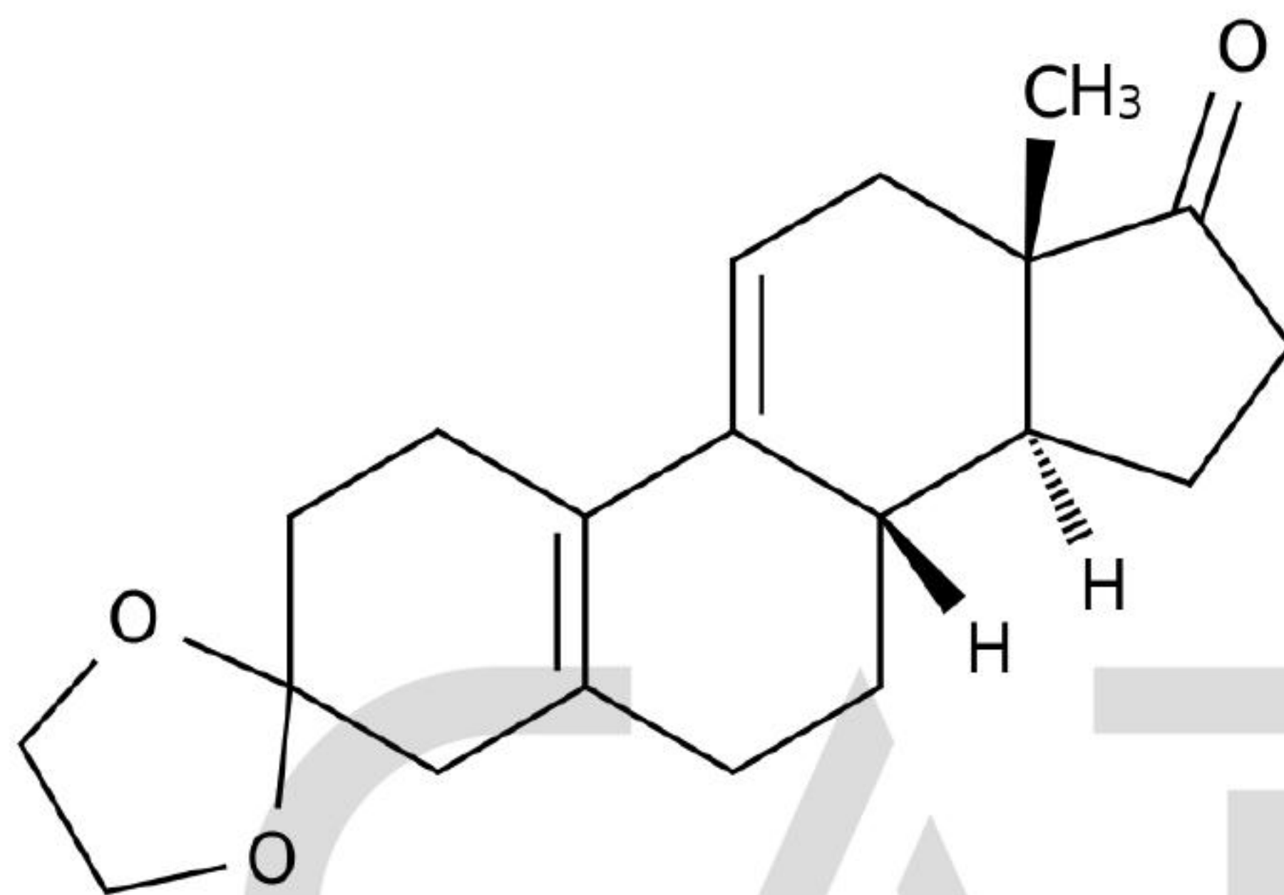
Chemical Structure:
