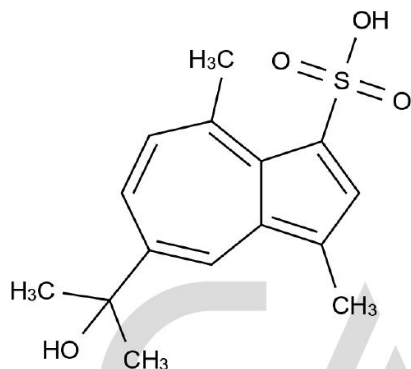
Chemical Structure:
