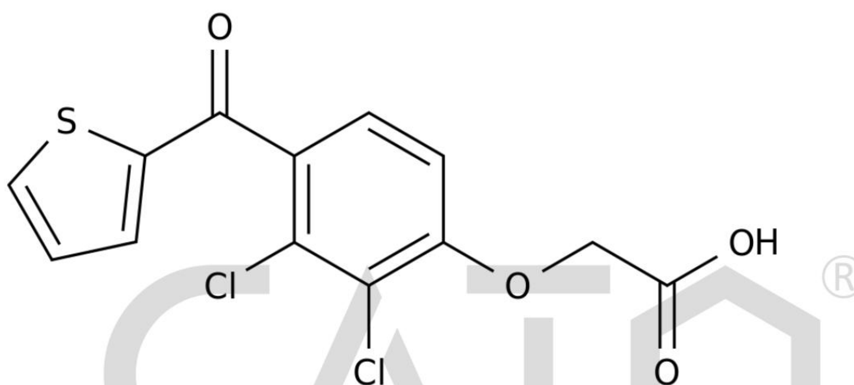
Chemical Structure:
