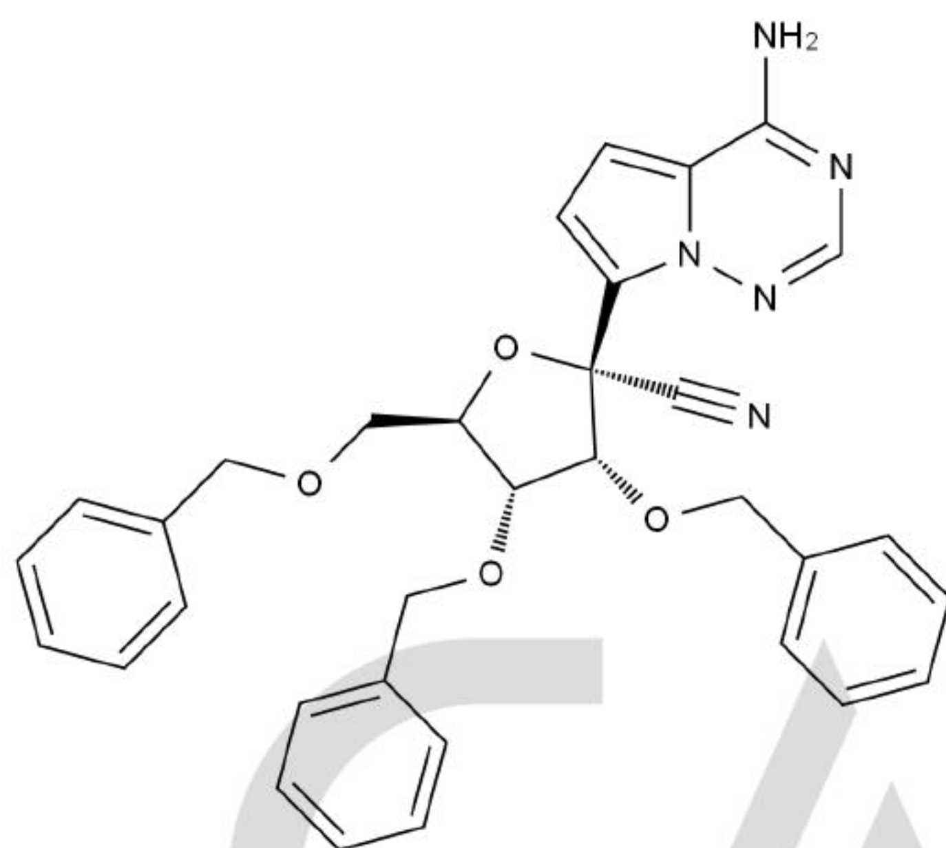
Chemical Structure:
