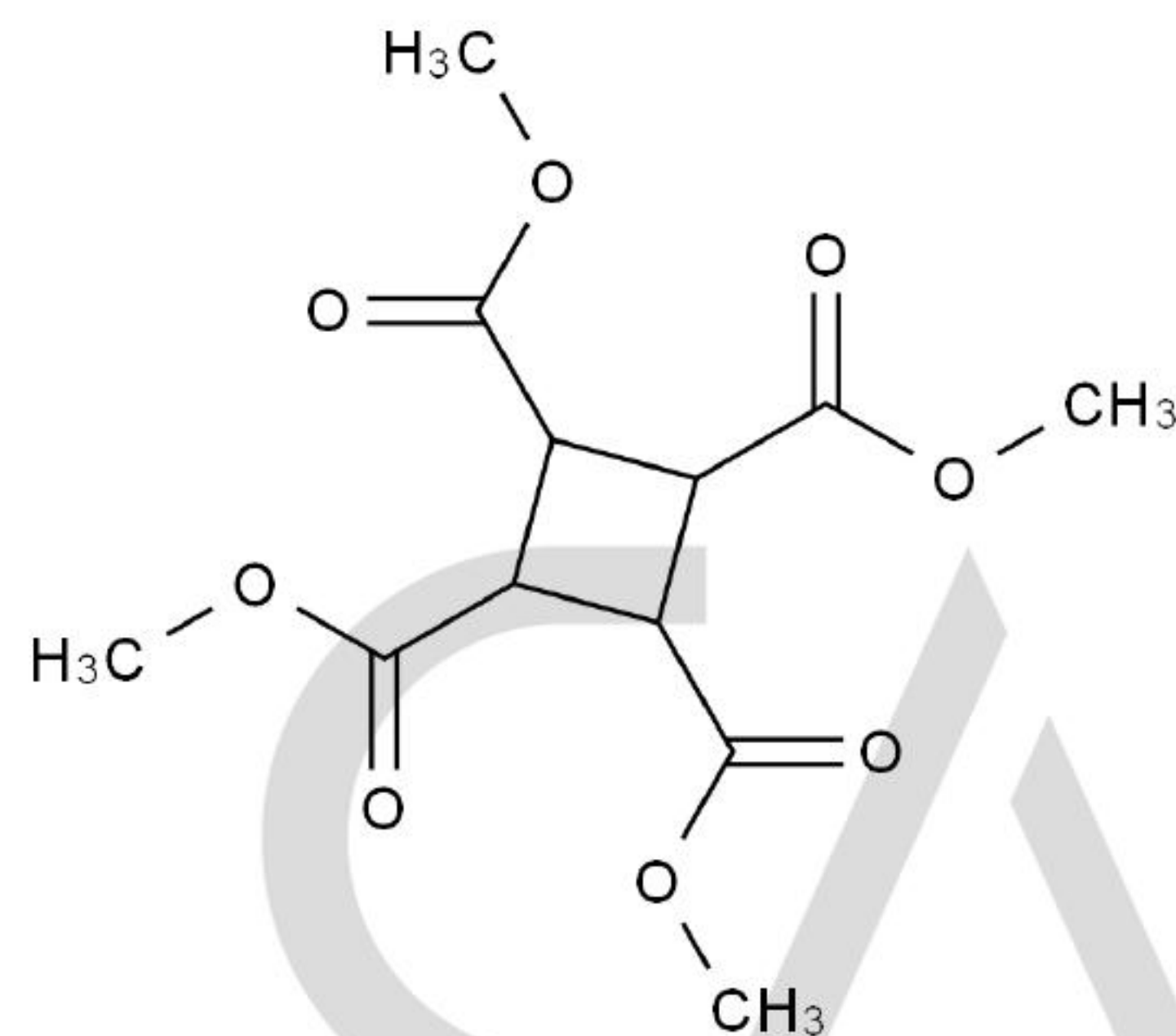
Chemical Structure:
