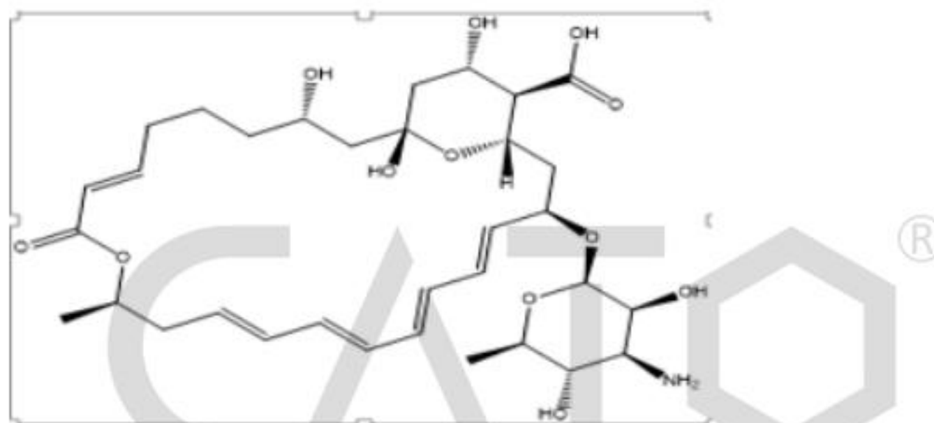
Chemical Structure:
