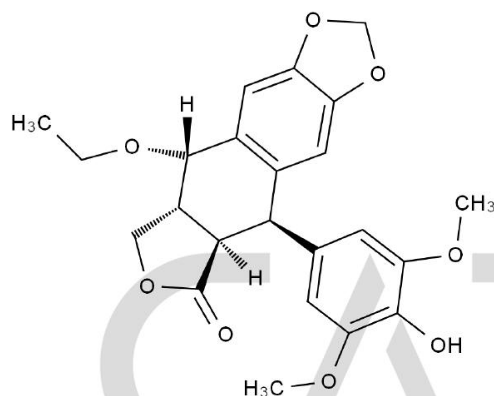
Chemical Structure:
