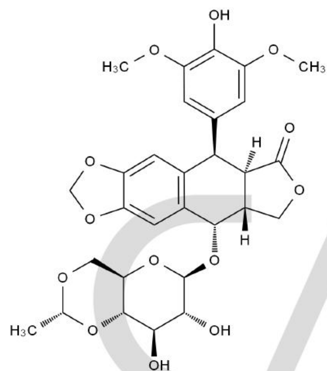
Chemical Structure:
