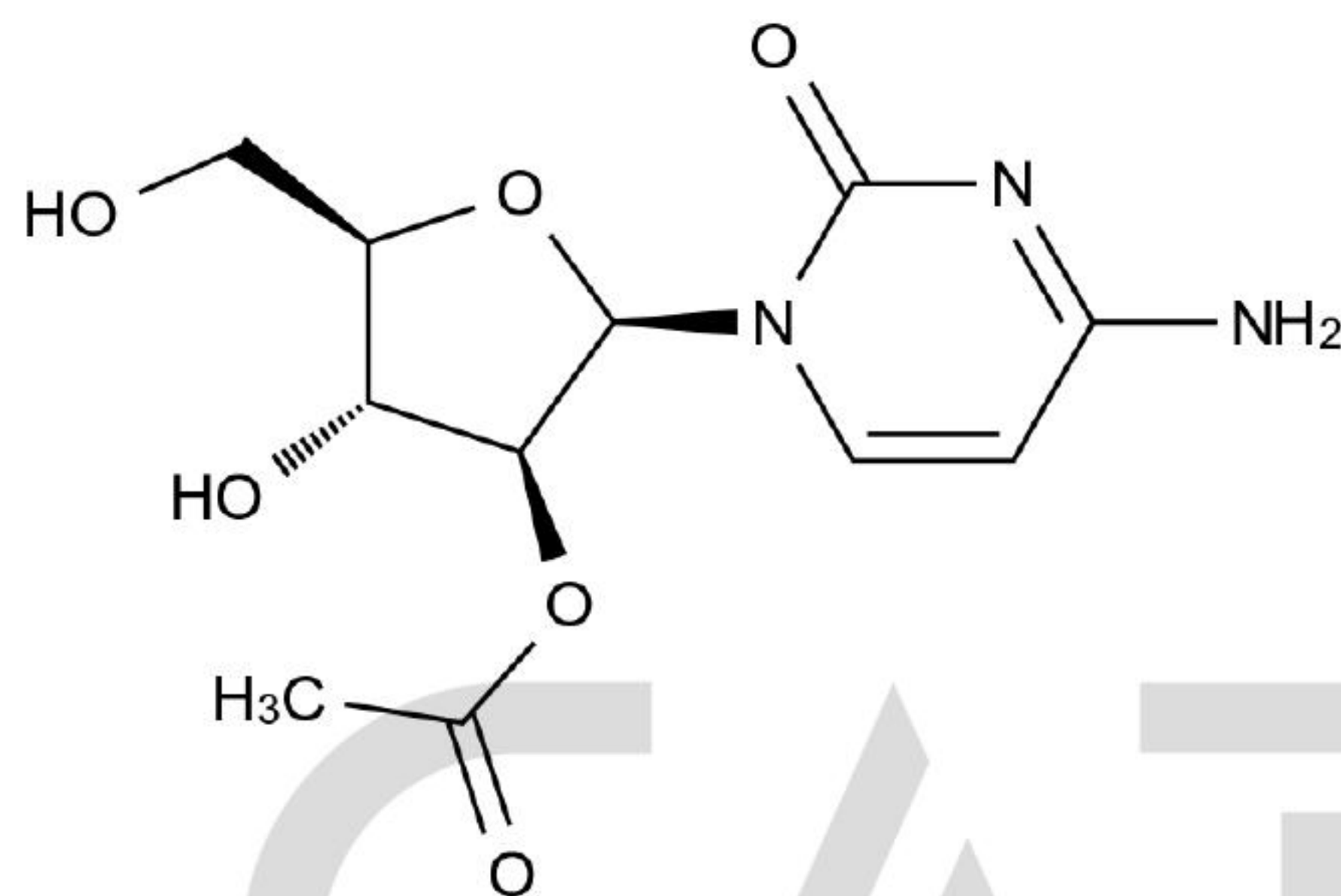
Chemical Structure:
