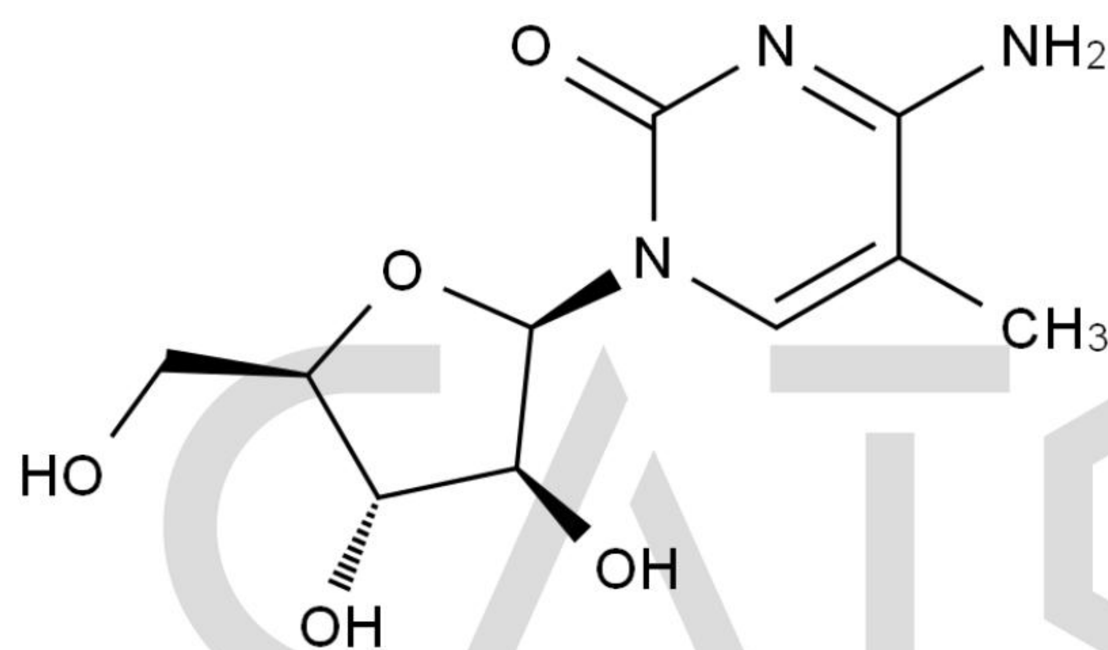
Chemical Structure:
