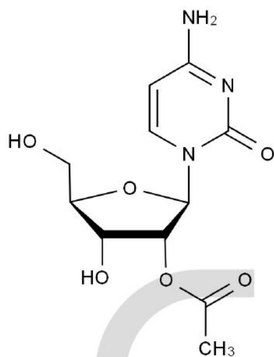
Chemical Structure:
