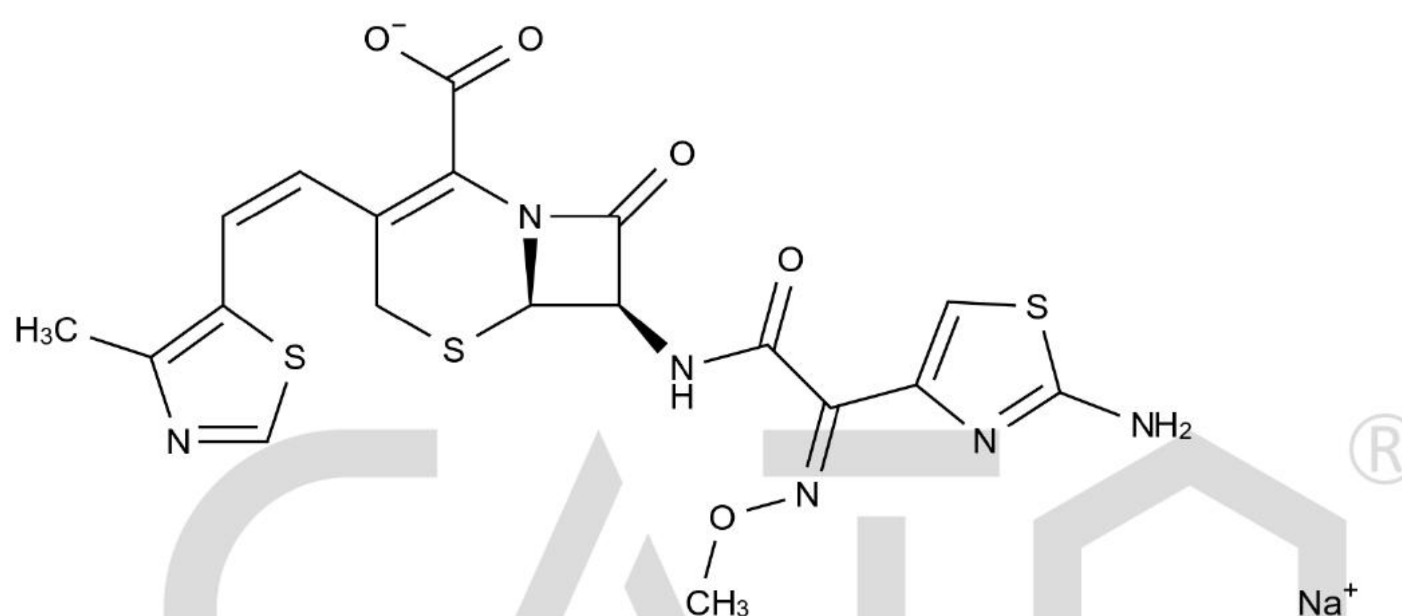
Chemical Structure:
