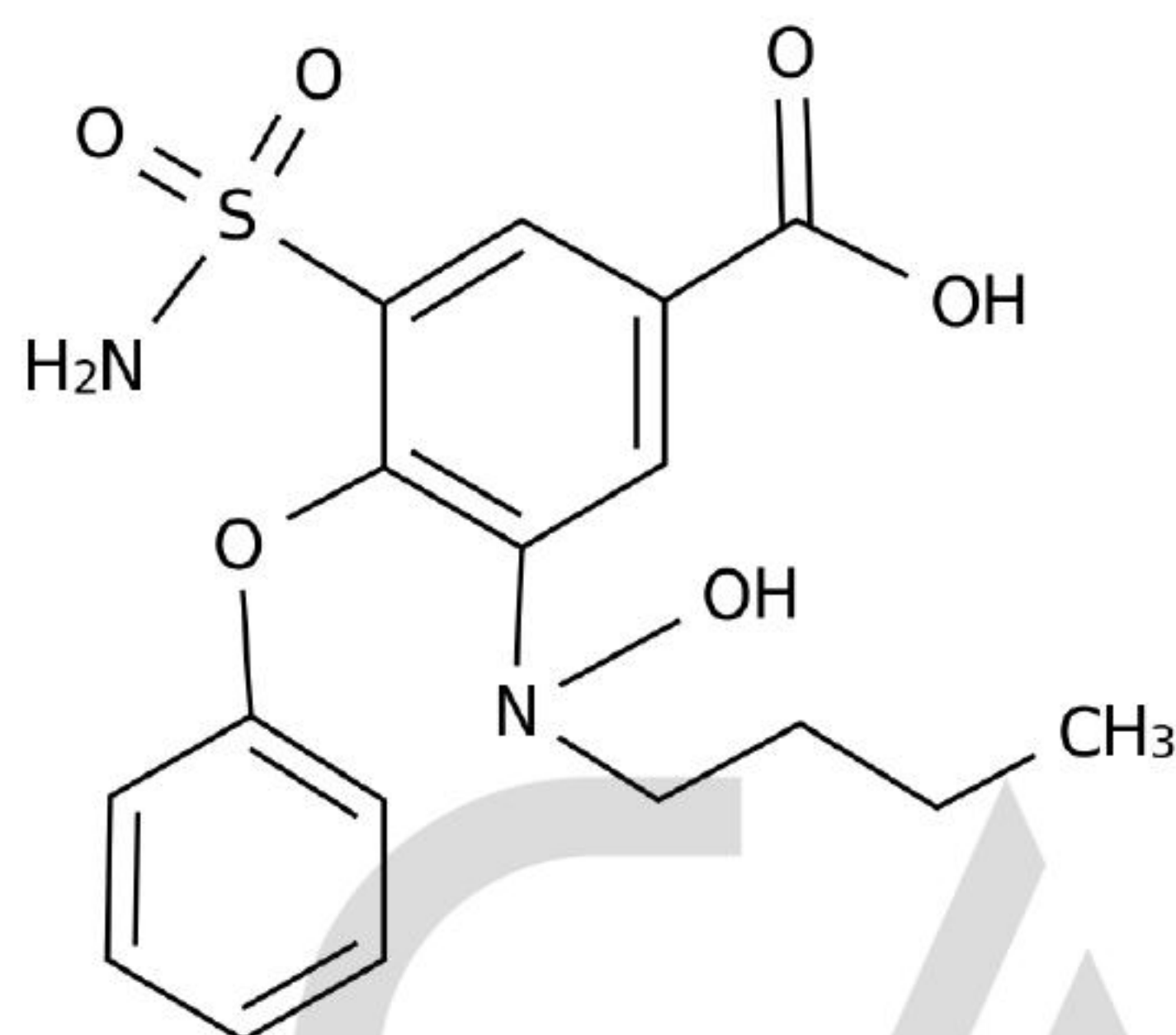
Chemical Structure:
