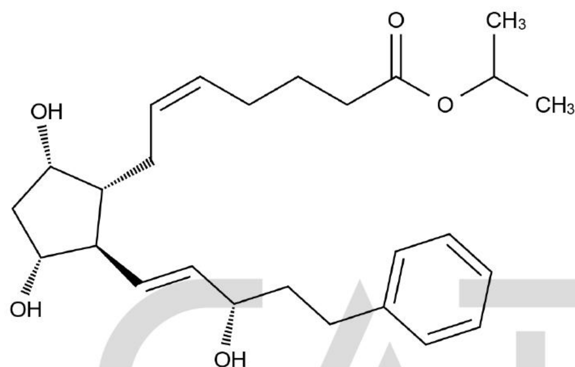
Chemical Structure:
