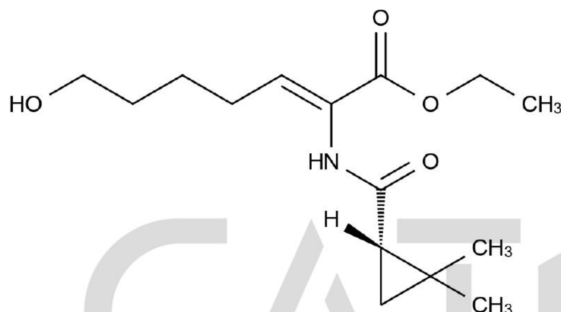
Chemical Structure:
