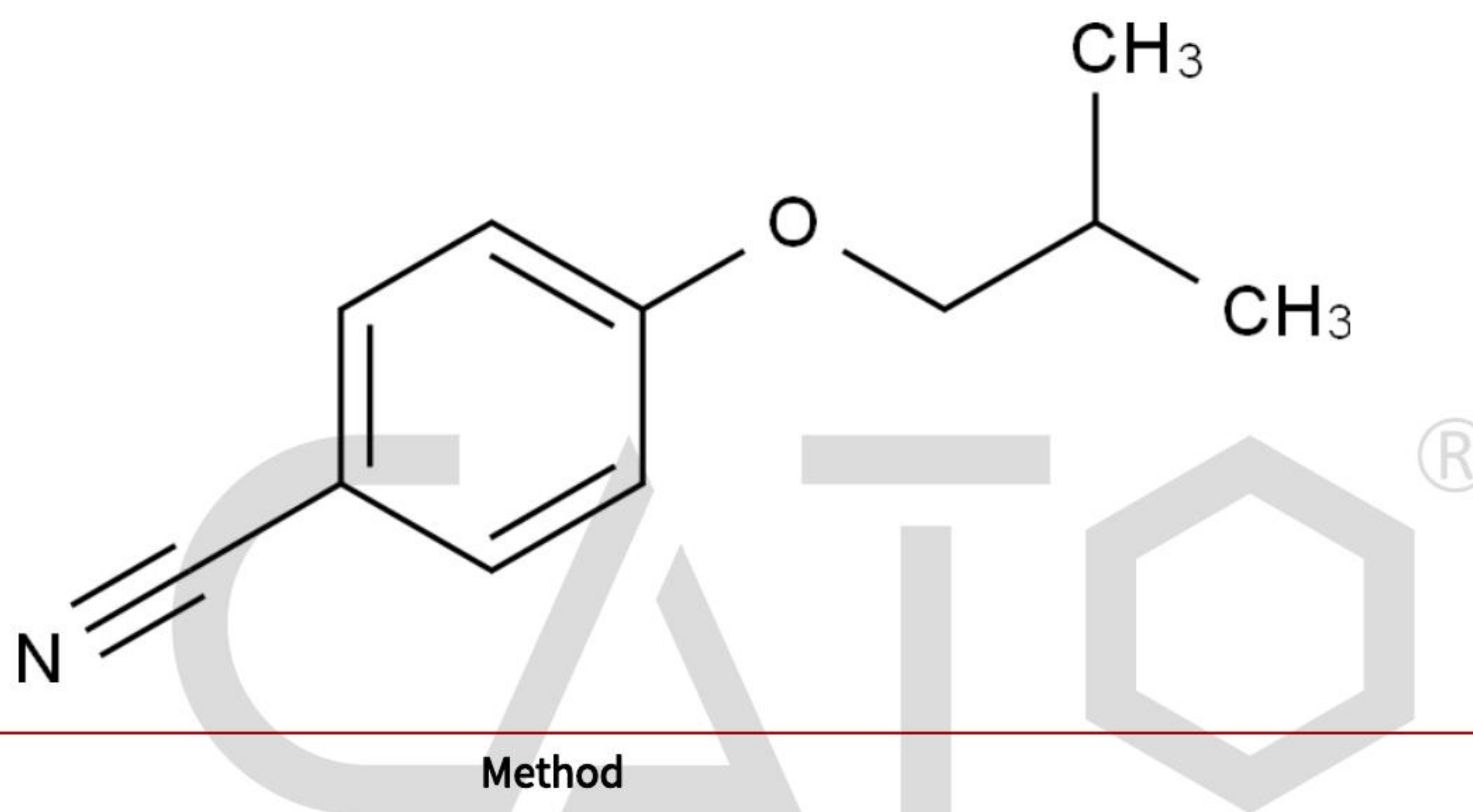
Chemical Structure:
