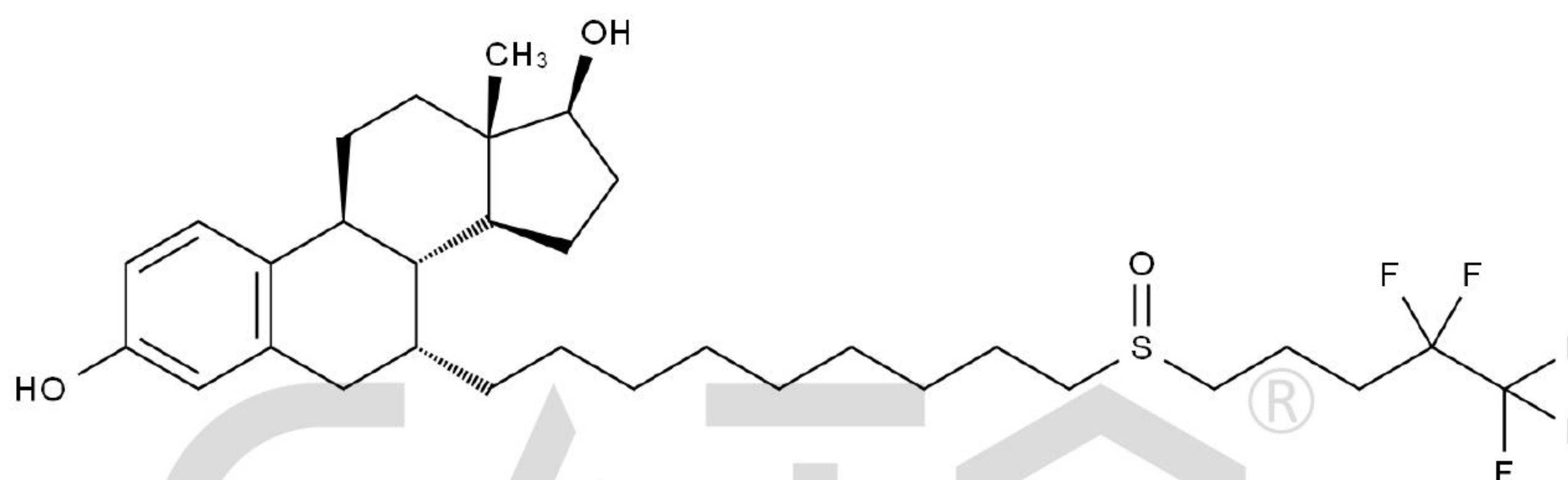
Chemical Structure:
