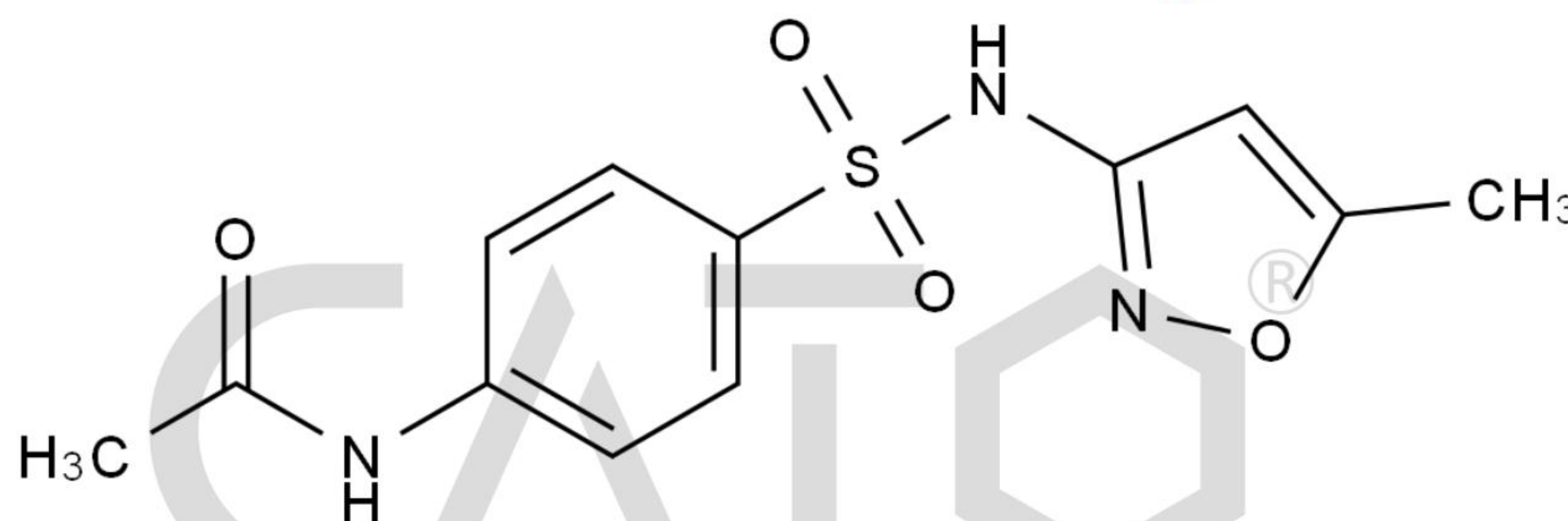
Chemical Structure:
