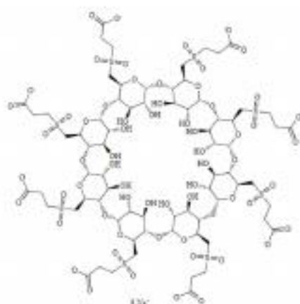
Chemical Structure:
