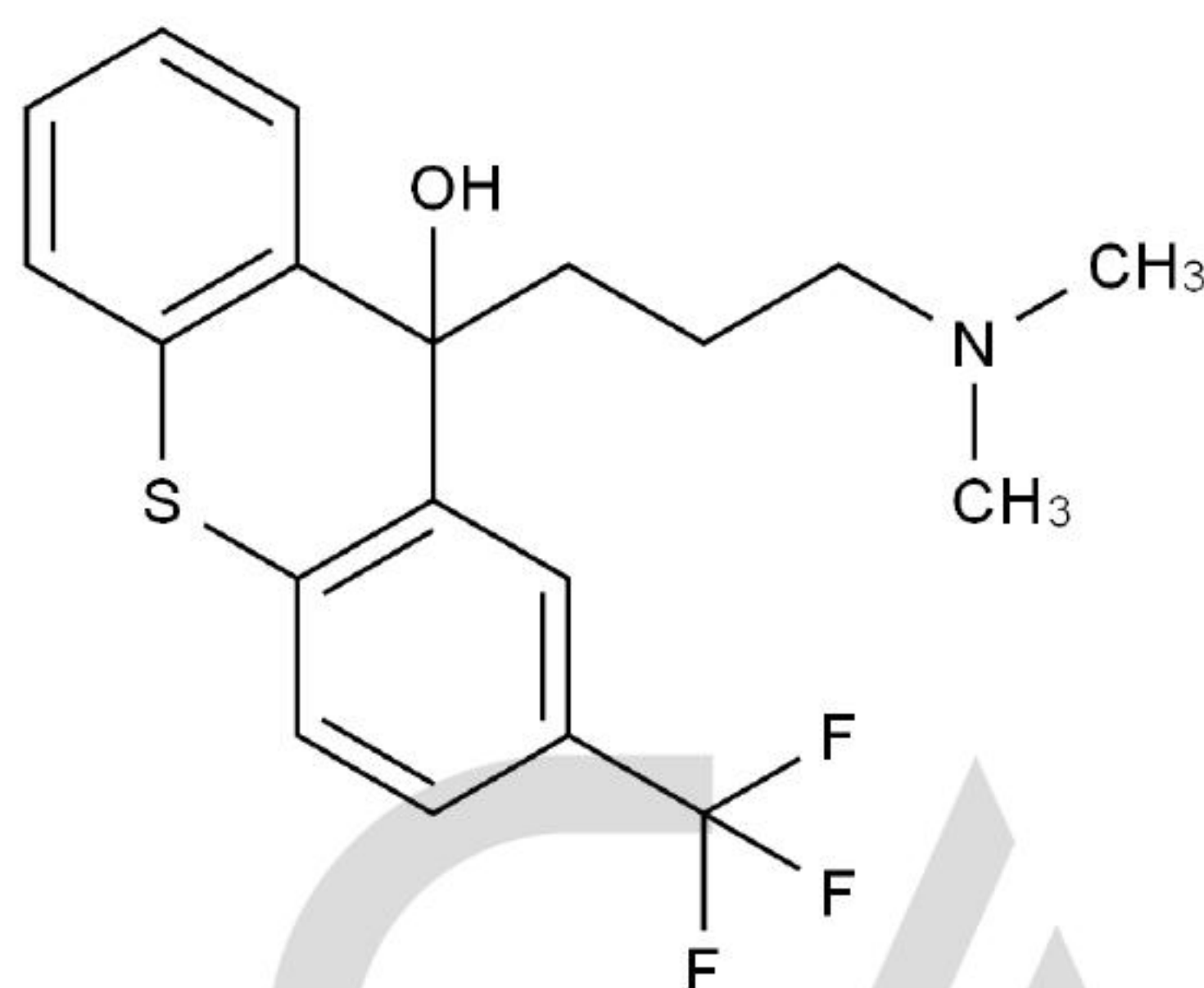
Chemical Structure:
