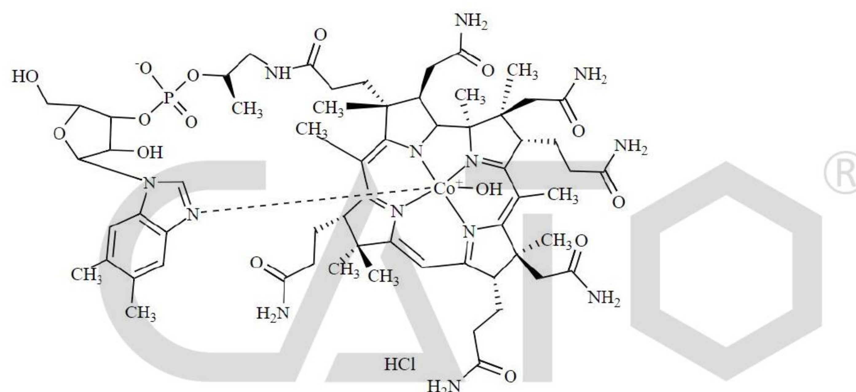
Chemical Structure:
