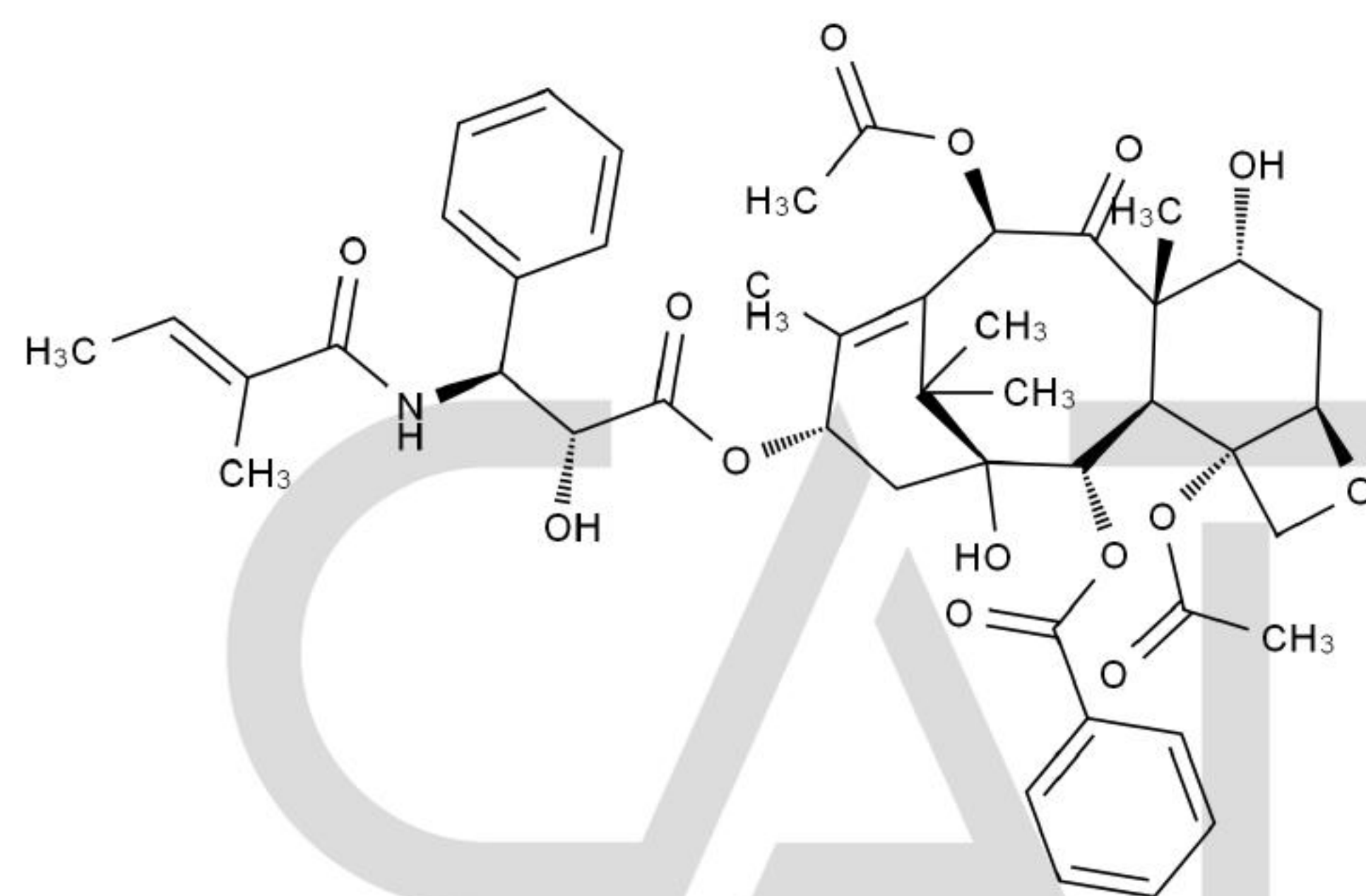
Chemical Structure:
