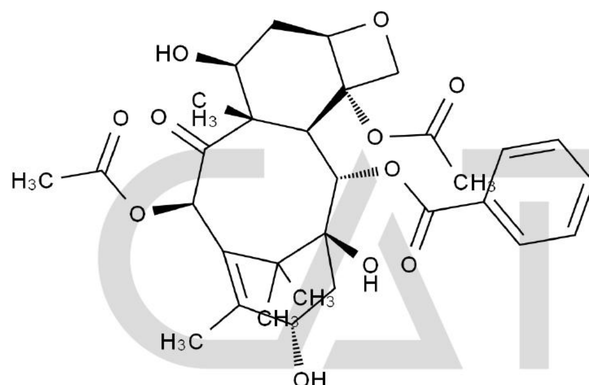
Chemical Structure:
