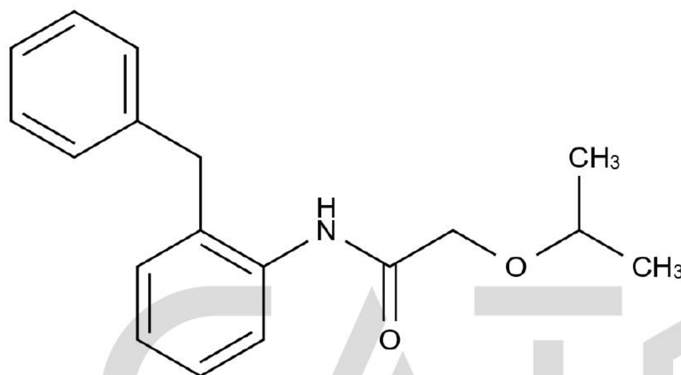
Chemical Structure:
