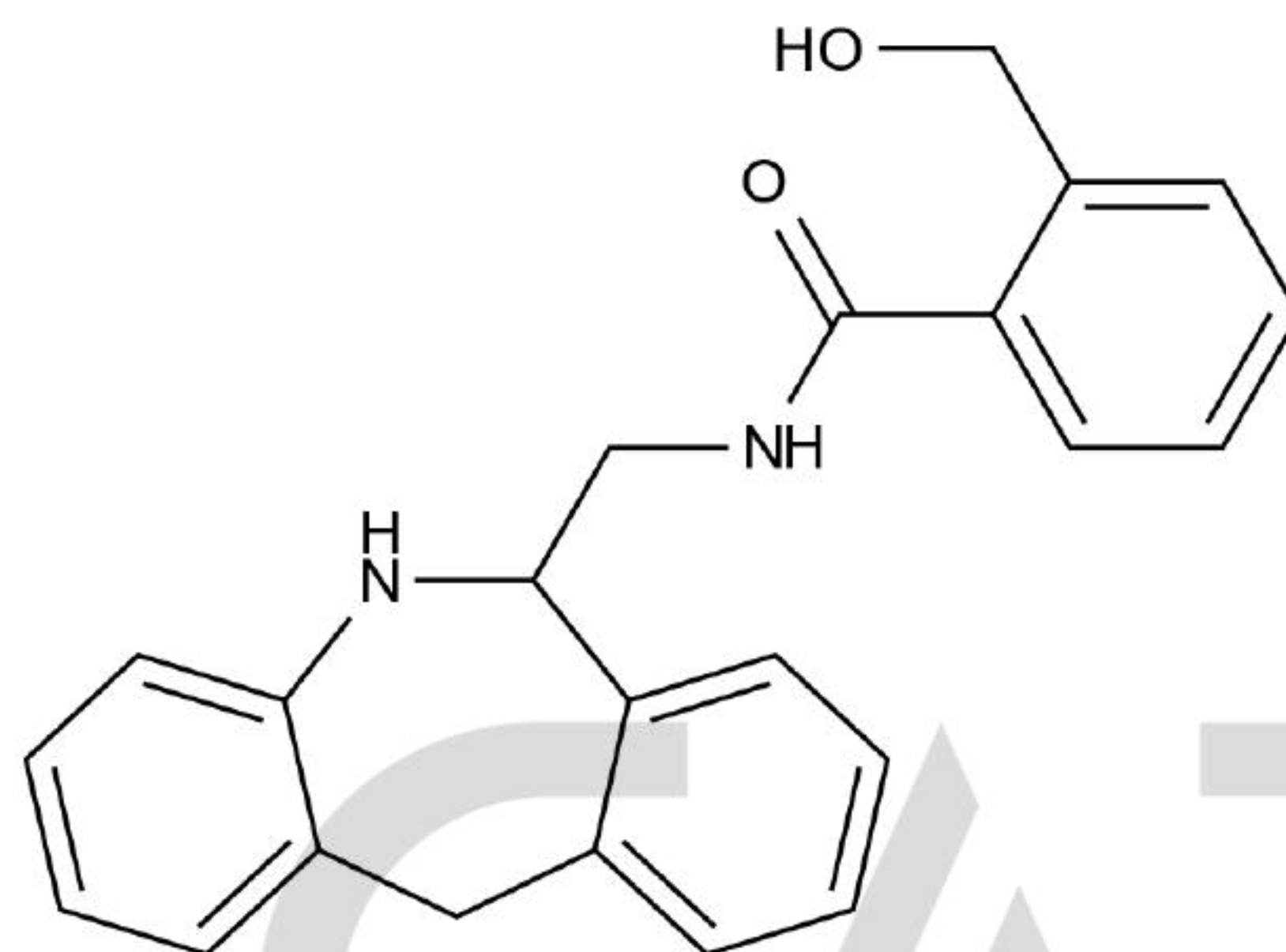
Chemical Structure:
