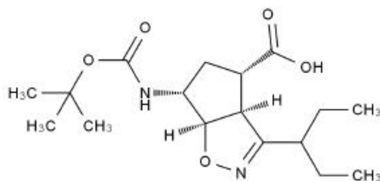
Chemical Structure:
