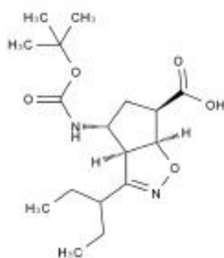
Chemical Structure:
