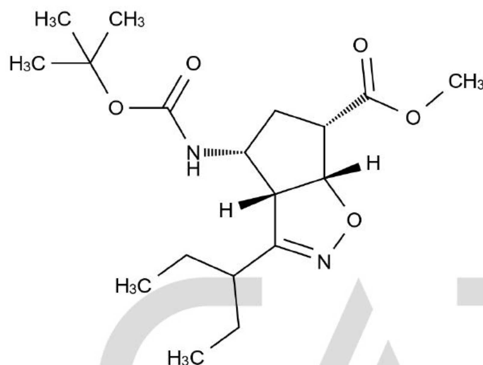
Chemical Structure:
