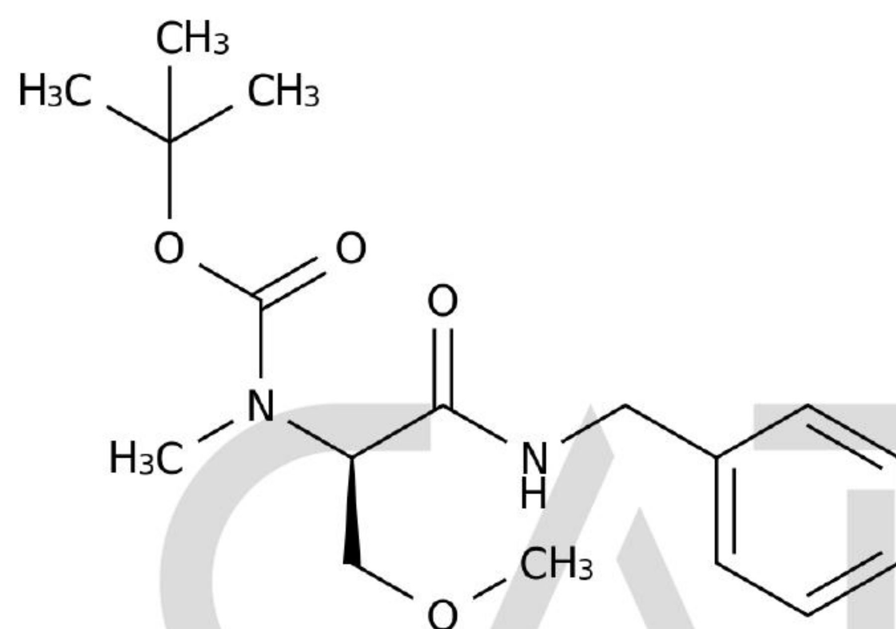
Chemical Structure:
