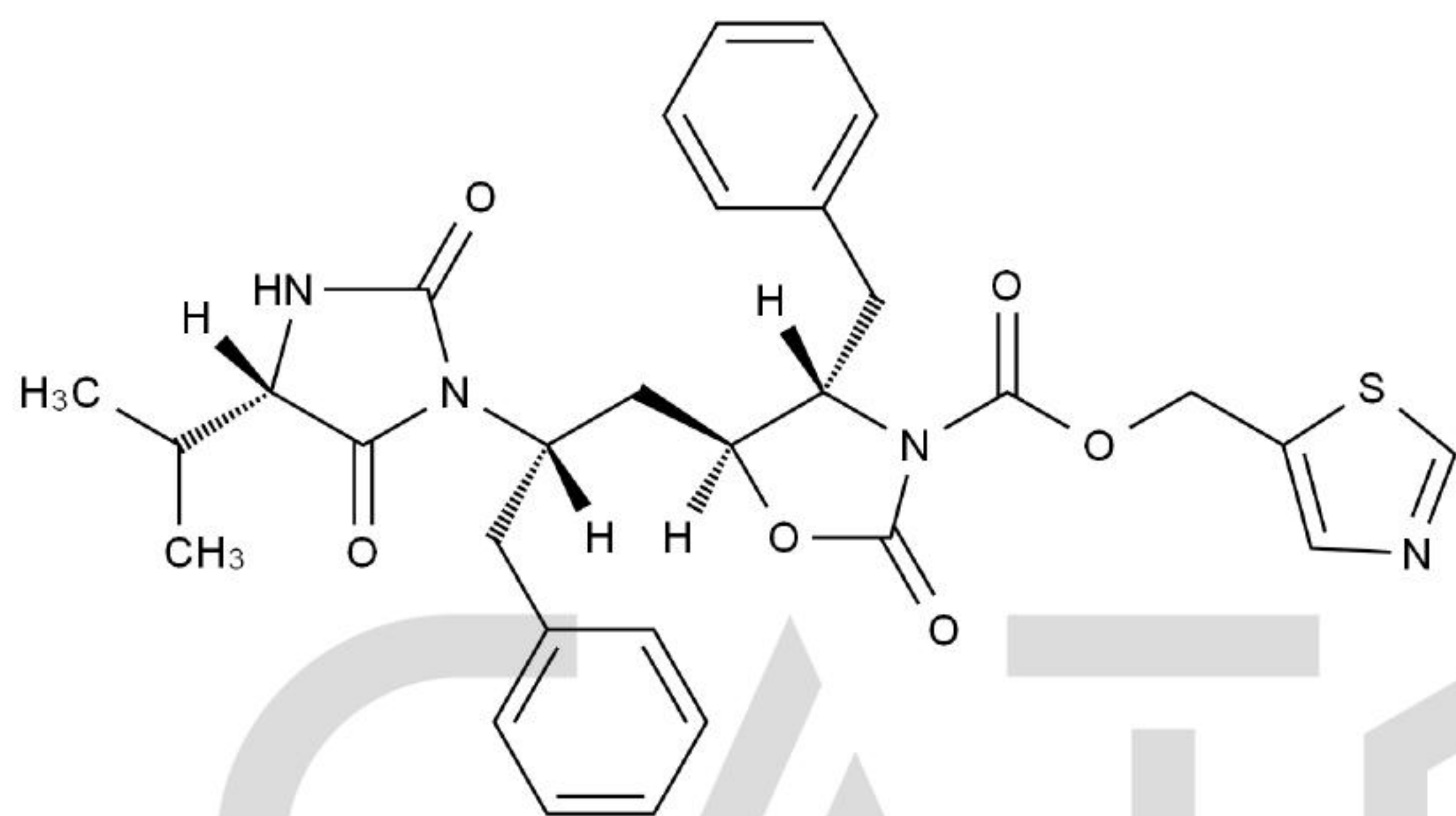
Chemical Structure:
