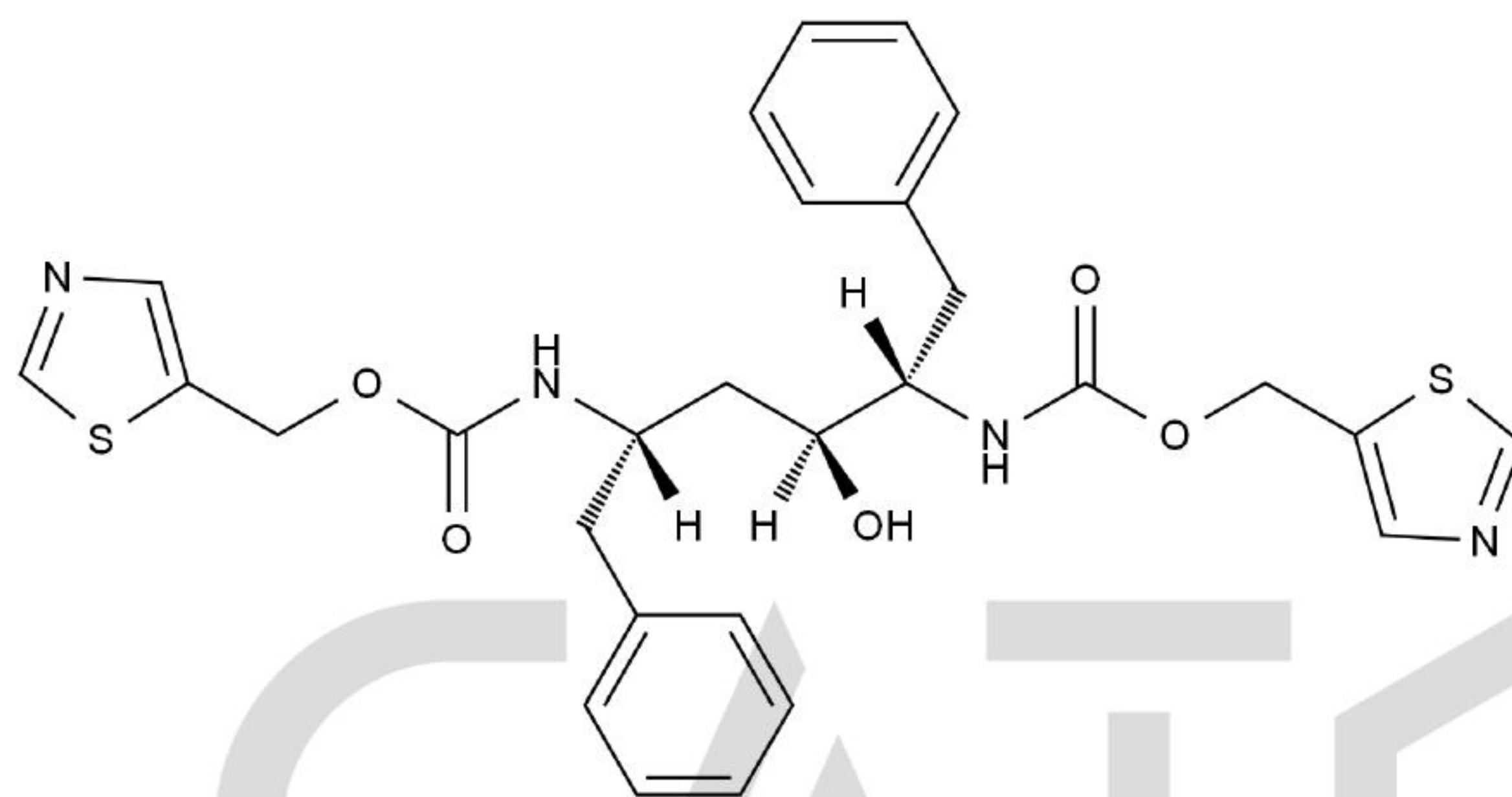
Chemical Structure:
