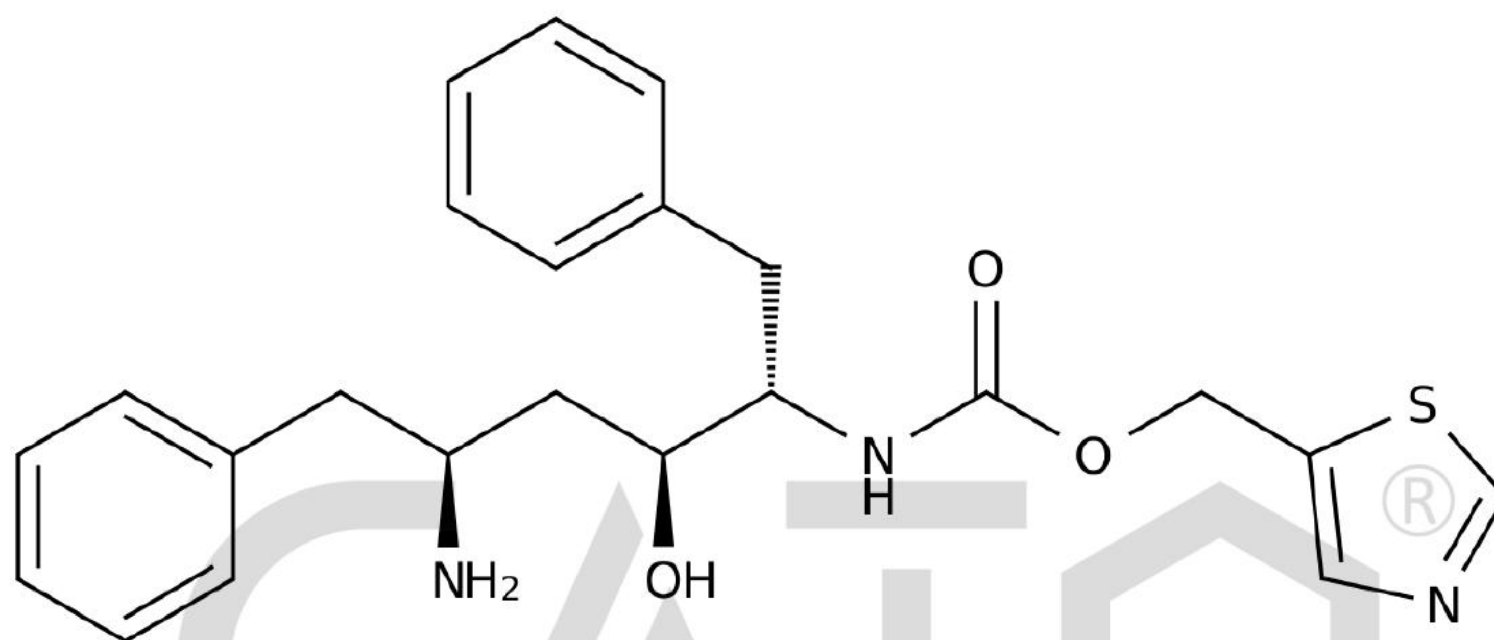
Chemical Structure:
