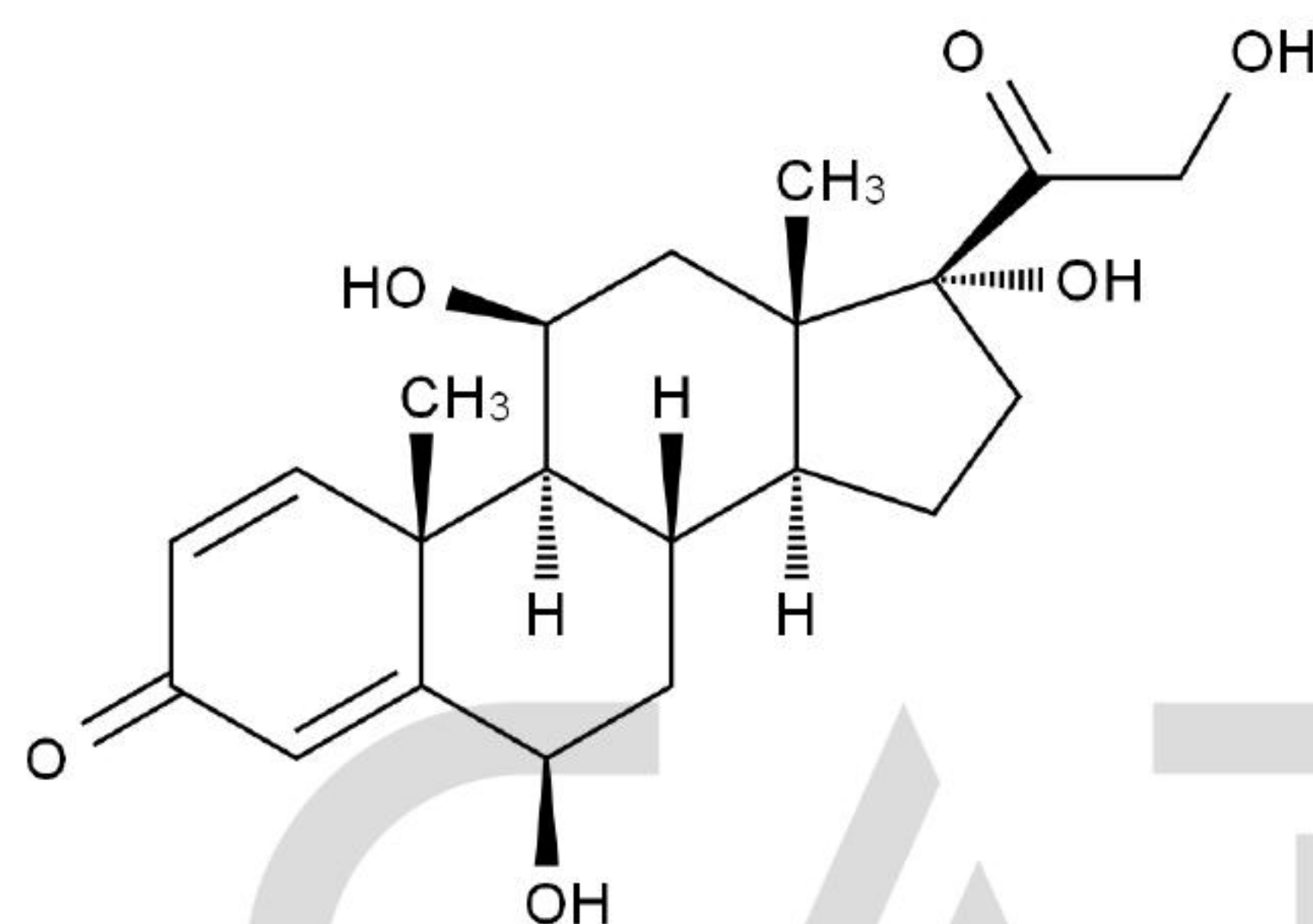
Chemical Structure:
