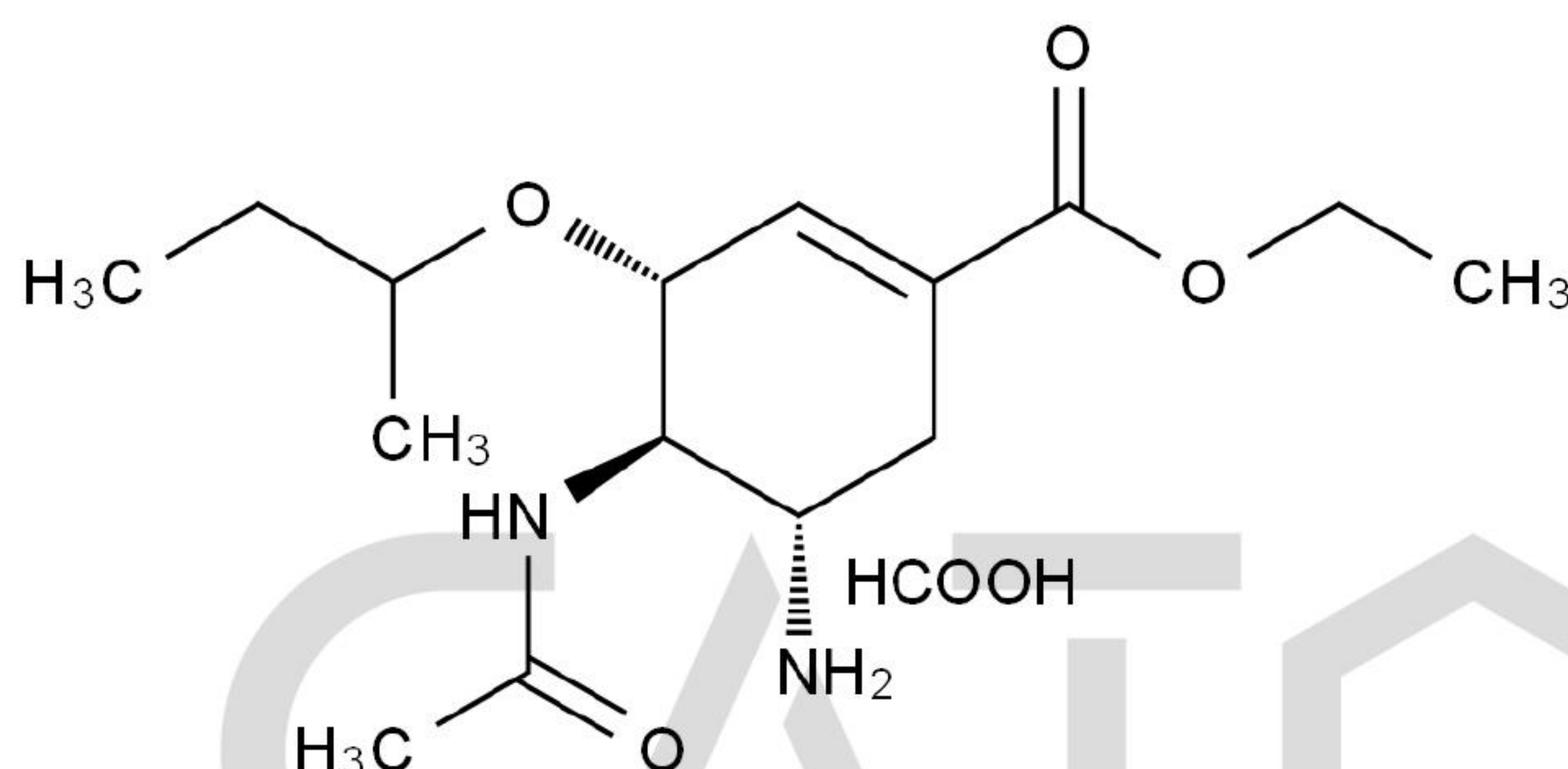
Chemical Structure:
