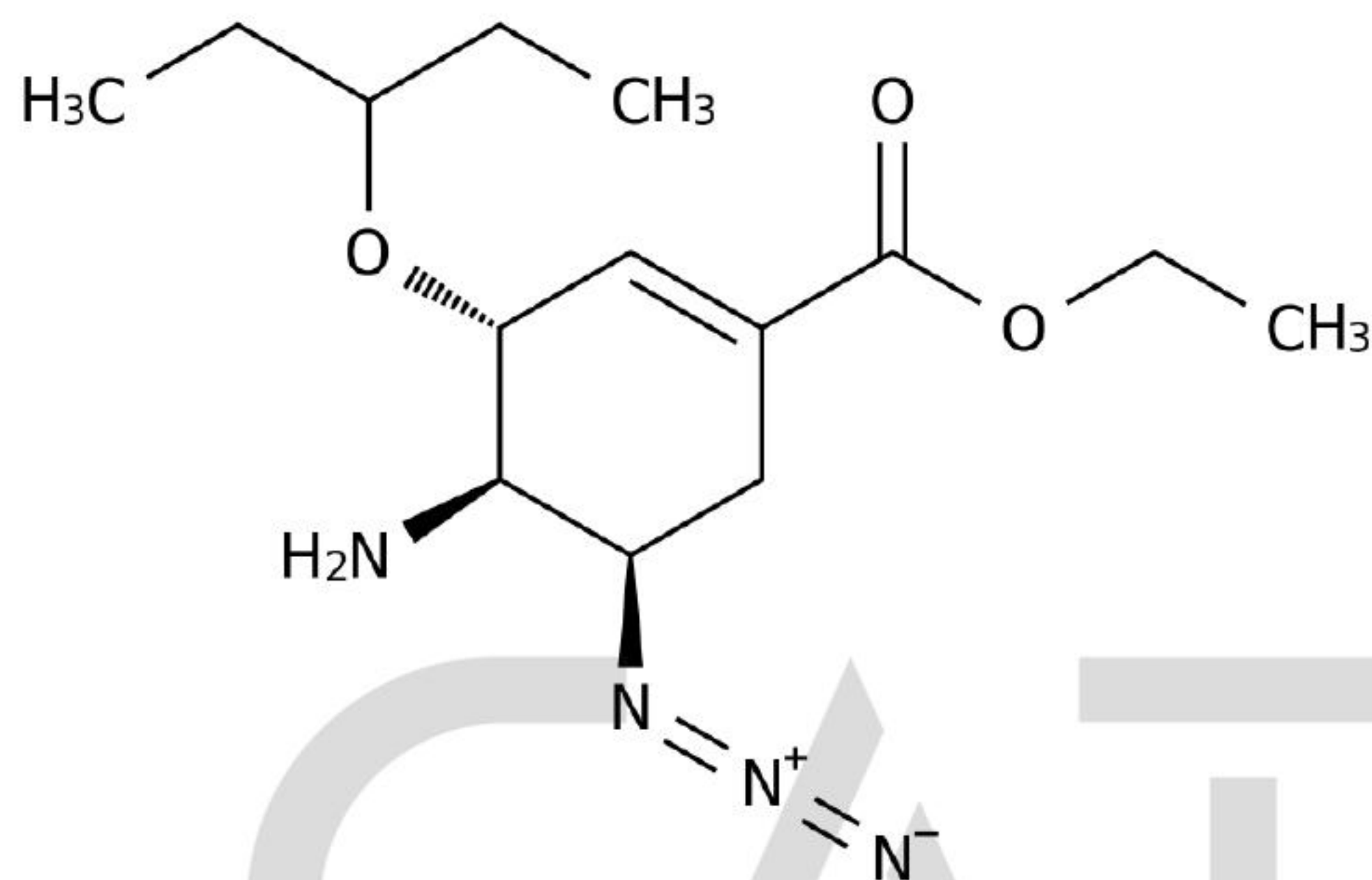
Chemical Structure:
