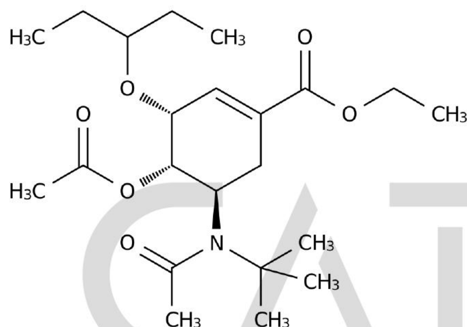
Chemical Structure:
