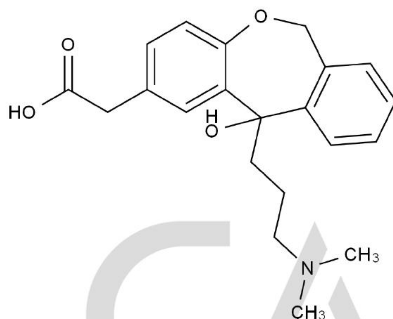
Chemical Structure:
