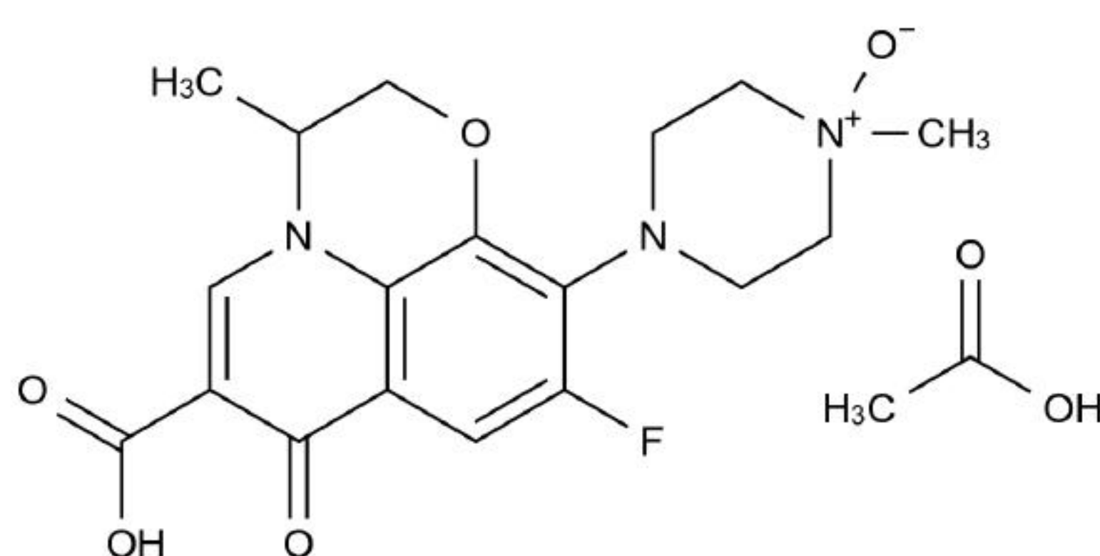
Chemical Structure:
