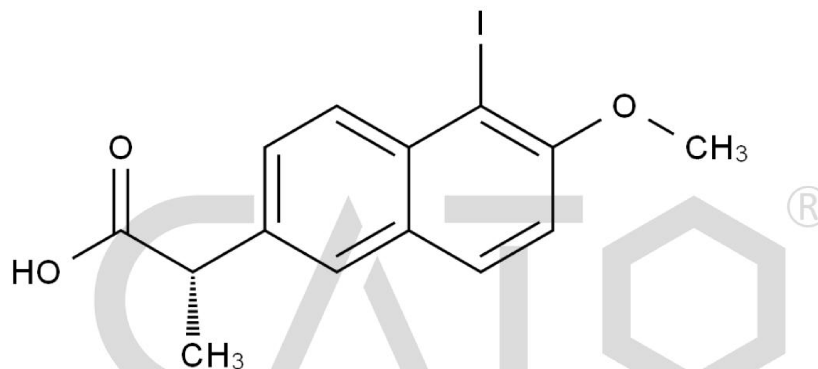
Chemical Structure:
