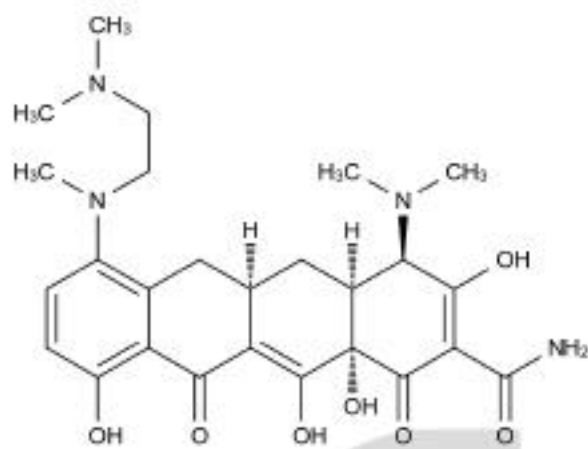
Chemical Structure:
